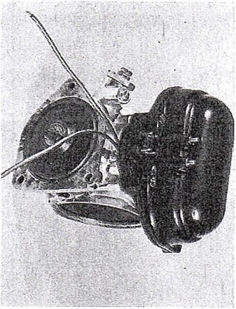
Place coil in proper location, checking to see that wires are not pinched between coil and case, also to see if carbon brushes are in proper location, and clearance for rotor is a sufficient distance from carbon brush housings.
