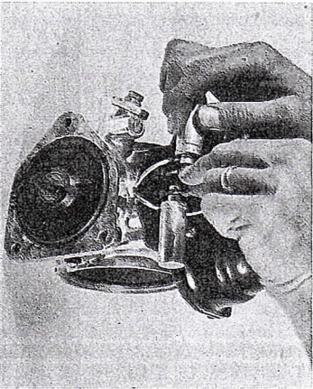
Form wires so they will fit between condensers and coil. Cut to proper length and solder wire terminal ends of appropriate size for condensers to ends of wires. Install Lincoln-Zephyr condensers with coil retaining screws firmly in place.
