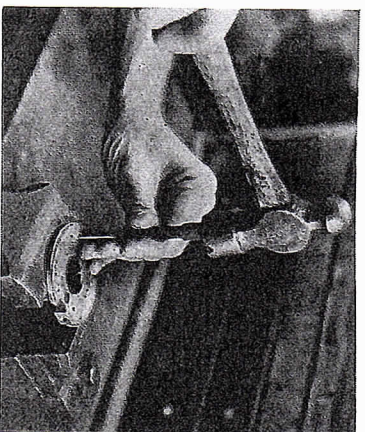
With drift punch remove the stock fulcrum pins and eccentric screws. Back the breaker plate up with the vise to prevent bending of plate.
