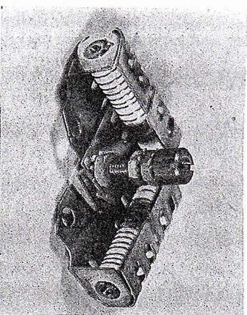
The Lincoln-Zephyr coil was manufactured for the use of resistance units, which in this case are two Ford coil resistors joined together as shown in photo to make up unit, which lets both coils get an equal amount of voltage. The main distributor lead is fastened to the center lug, which joins the resistors. Unit is fastened to coil by using two 8/32 nuts.
