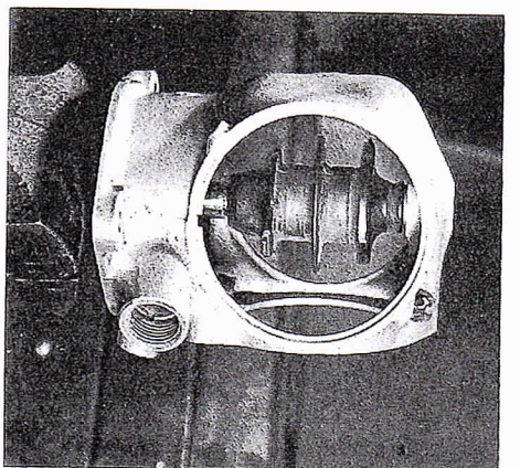
With the inserting of the Lincoln Zephyr rotor on the new rotor location, on the Ford distributor shaft and then inserting the shaft into the Ford base, insert the assembled unit into the Lincoln case.
